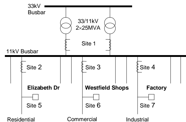
Fig. 3: Layout of Test Area
