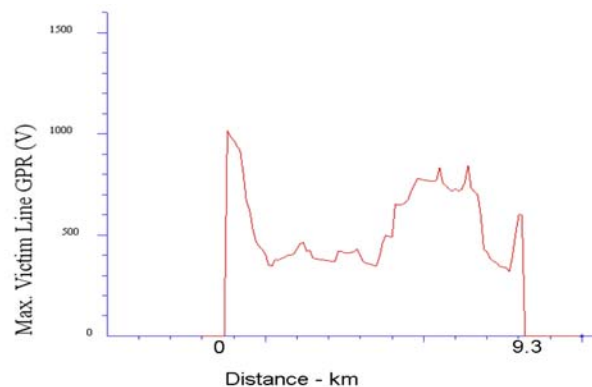
Figure 6: Inductive Coating Stress Voltage with gradient control wire
