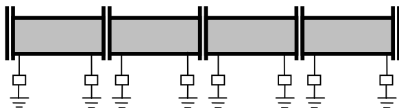
Figure 1: Use of insulating joints
