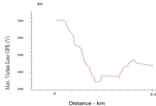
Figure 4: Inductive Coating Stress Voltage with no mitigation applied
