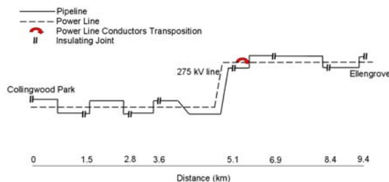
Figure 3: Physical layout of a Brisbane shared corridor
