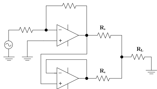
Figure 4: Parallelisation of power op-amps
