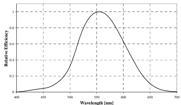
Figure 2: CEI Spectral luminous efficiency curve
