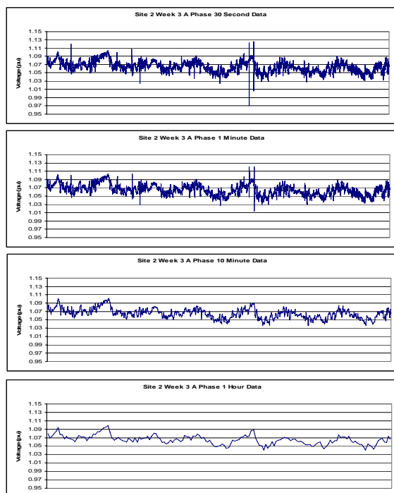
Figure 3.1: One Week Voltage Trend for Site 5; Data Aggregated to 30 Second, 1 Minute, 10 Minute and 1 Hour Intervals
