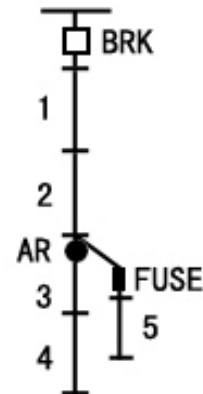
Figure 3 Topology of a Simple Feeder with AR
