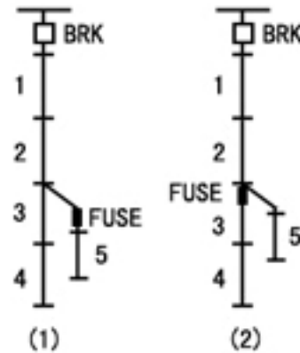
Figure 2 Topology of a Simple Feeder
