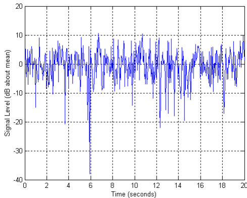
Figure 8. Fading pattern for transmit antenna at position E in the lecture theatre.
