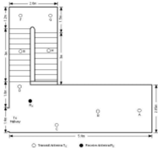
Figure 3. Floor plan and antenna placements for the stairwell.
