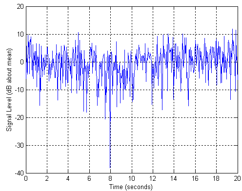
Figure 6. Fading pattern for transmit antenna at position C in the hallway.
