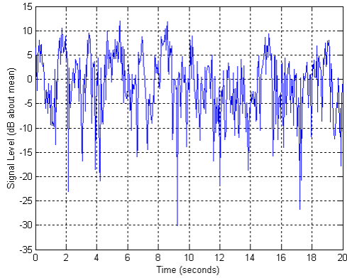
Figure 7. Fading pattern for transmit antenna at position E in the stairwell.
