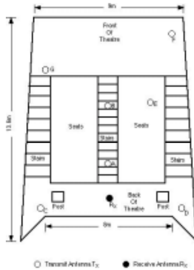
Figure 4. Floor plan and antenna placements for the lecture theatre.
