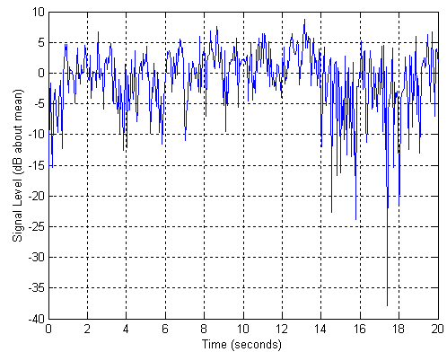
Figure 5. Fading pattern for transmit antenna at position B in the small room.
