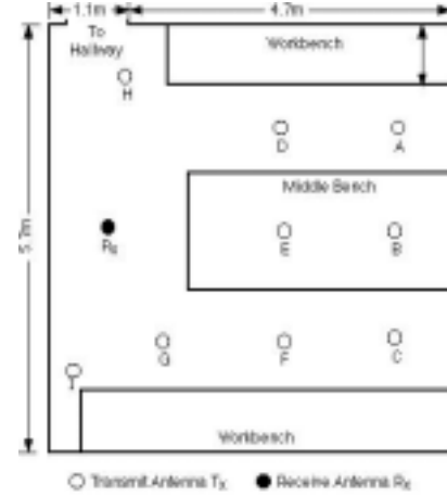
Figure 1. Floor plan and antenna placements for the small room.
